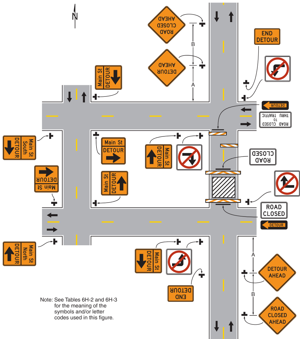
Typical Application 20
